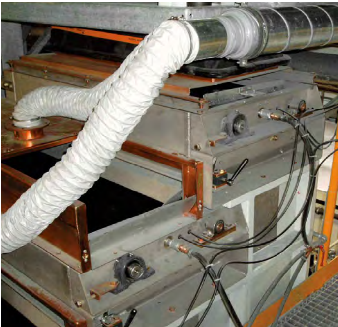
Hochintensitätsscheider 2-stufig High intensity separator, two-staged design
